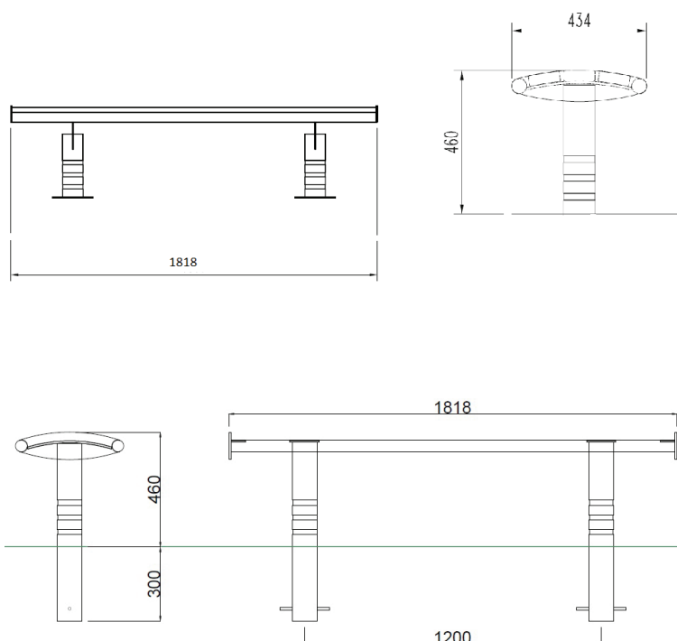
Image shows Wessex Bench in RAL 9007, Below Ground Fix, with optional arm rests
